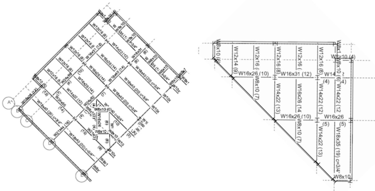
Figure 4: Existing Framing Sections (Floor on left, Wing on right)
