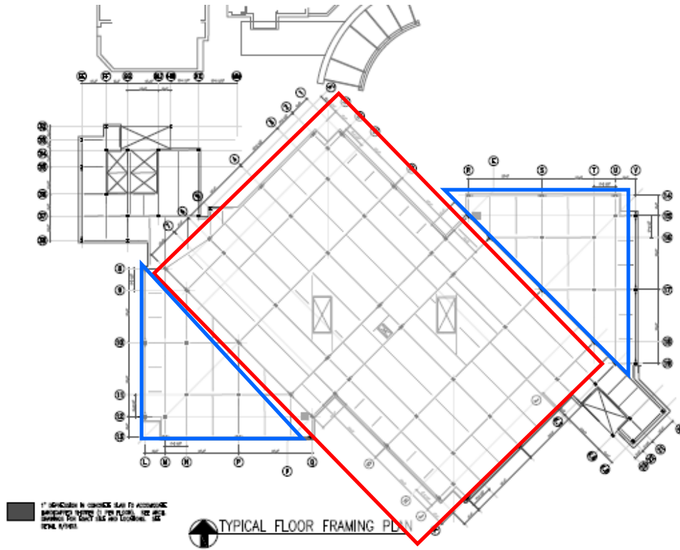
Figure 3: Framing Sections (Floor in Red, Wings in Blue)
